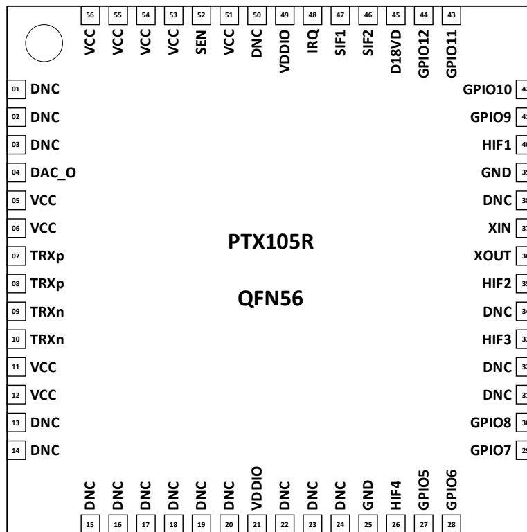
Figure 2: Pin Diagram
