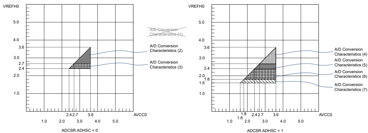
Figure 2.60 AVCC0 to VREFH0 voltage range
