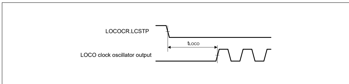
Figure 2.7 LOCO clock oscillation start timing
