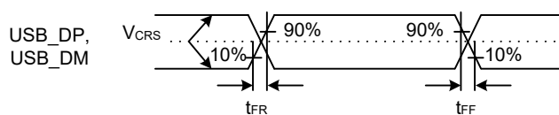
Figure 2.58 USB_DP and USB_DM output timing in full-speed mode
