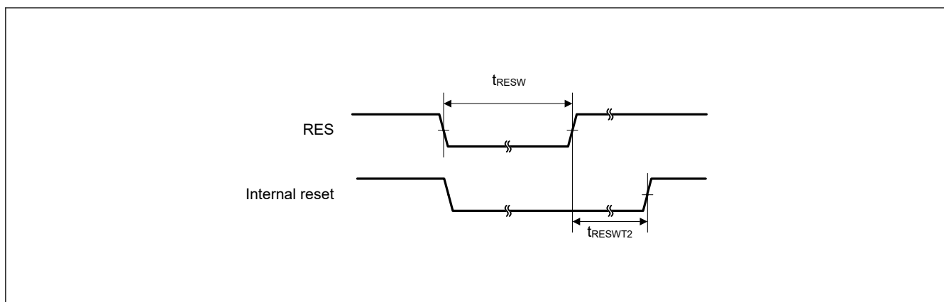
Figure 2.12 Reset input timing (1)
