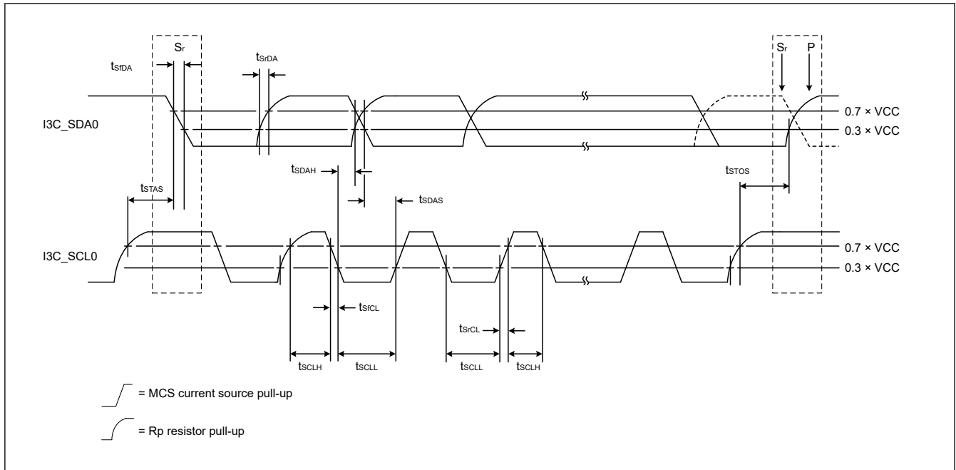
Figure 2.42 I²C bus interface input/output timing (Hs-mode)
