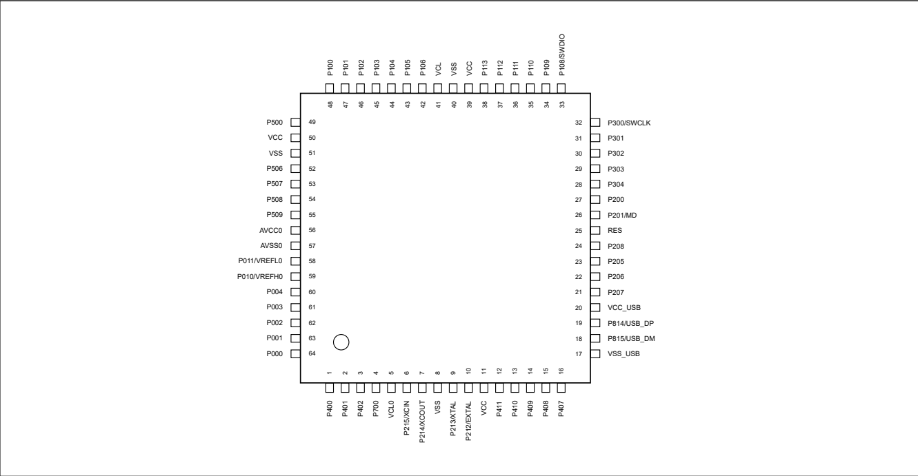
Figure 1.6 Pin assignment for LQFP 64-pin
