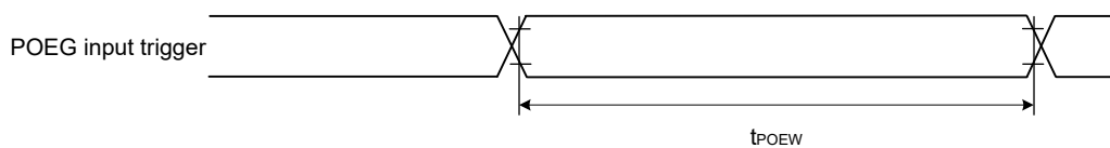
Figure 2.19 POEG input trigger timing
