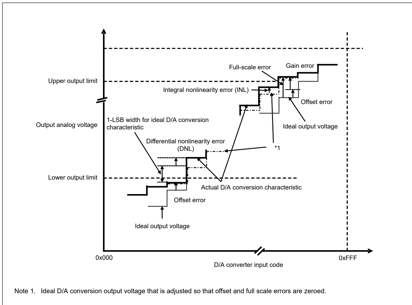
Figure 2.63 Illustration of D/A converter characteristic terms
