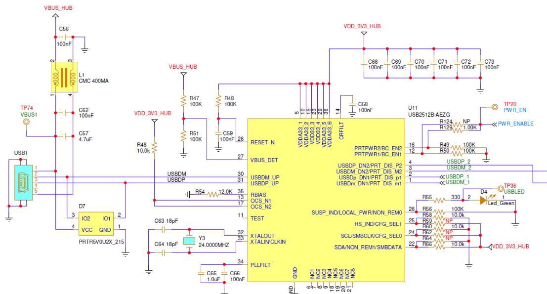
Figure 23. USB HUB circuitry
