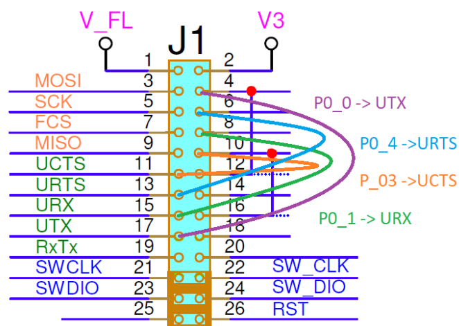
Figure 46. Enable two-wire UART with jumper wires
